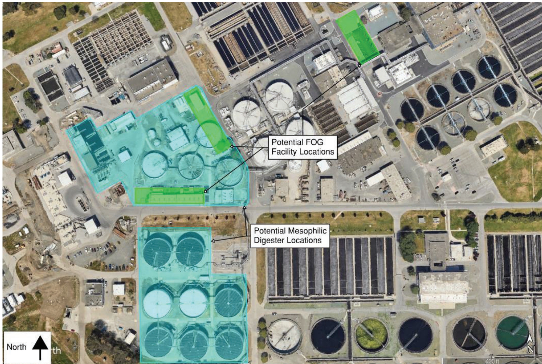
Figure 1-2 RWF Site Plan – Existing Site and Potential Locations of ADFU Project Elements
