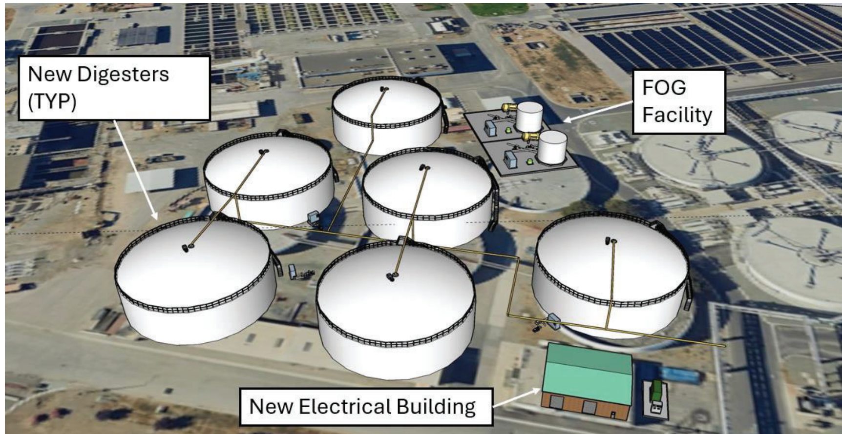
Figure 1-9 Indicative Design 3 – Alternative 2 2045 3D Layout
