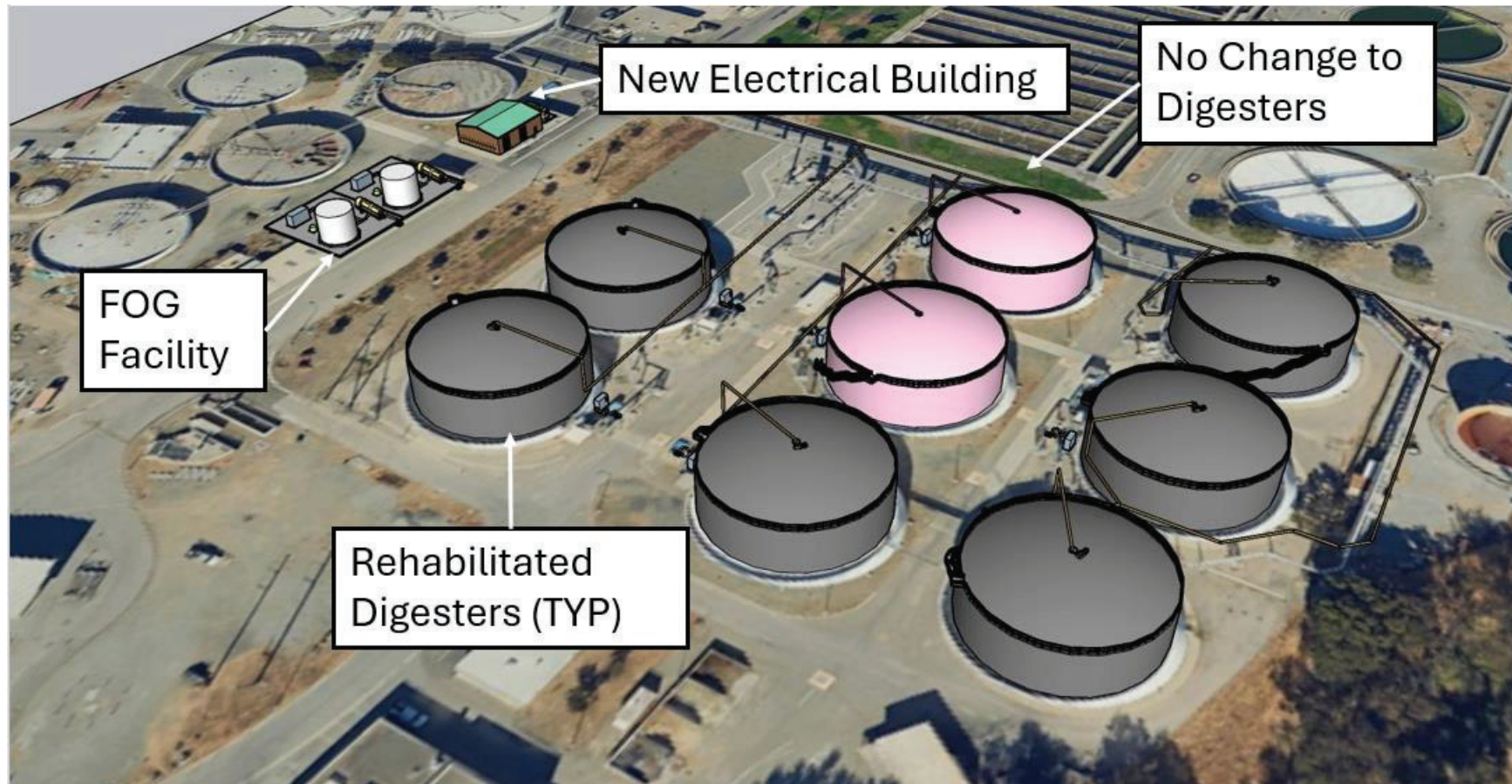
Figure 1-5 Indicative Design 1 – Base Alternative 2045 3D Layout
