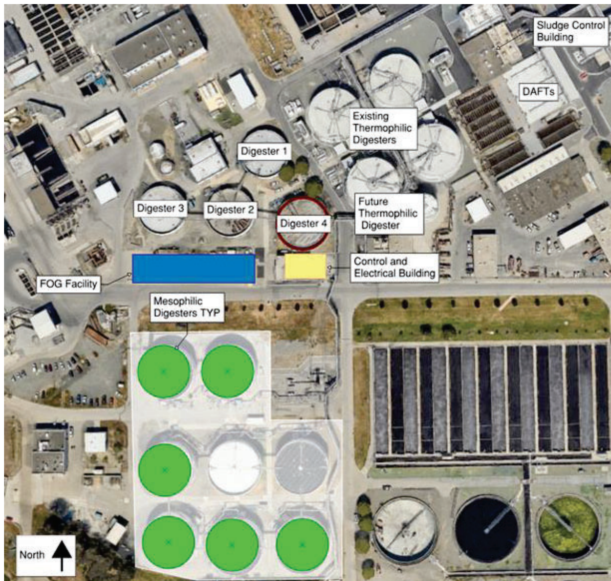
Figure 1-6 Indicative Design 2 – Alternative 1 2045 Layout
