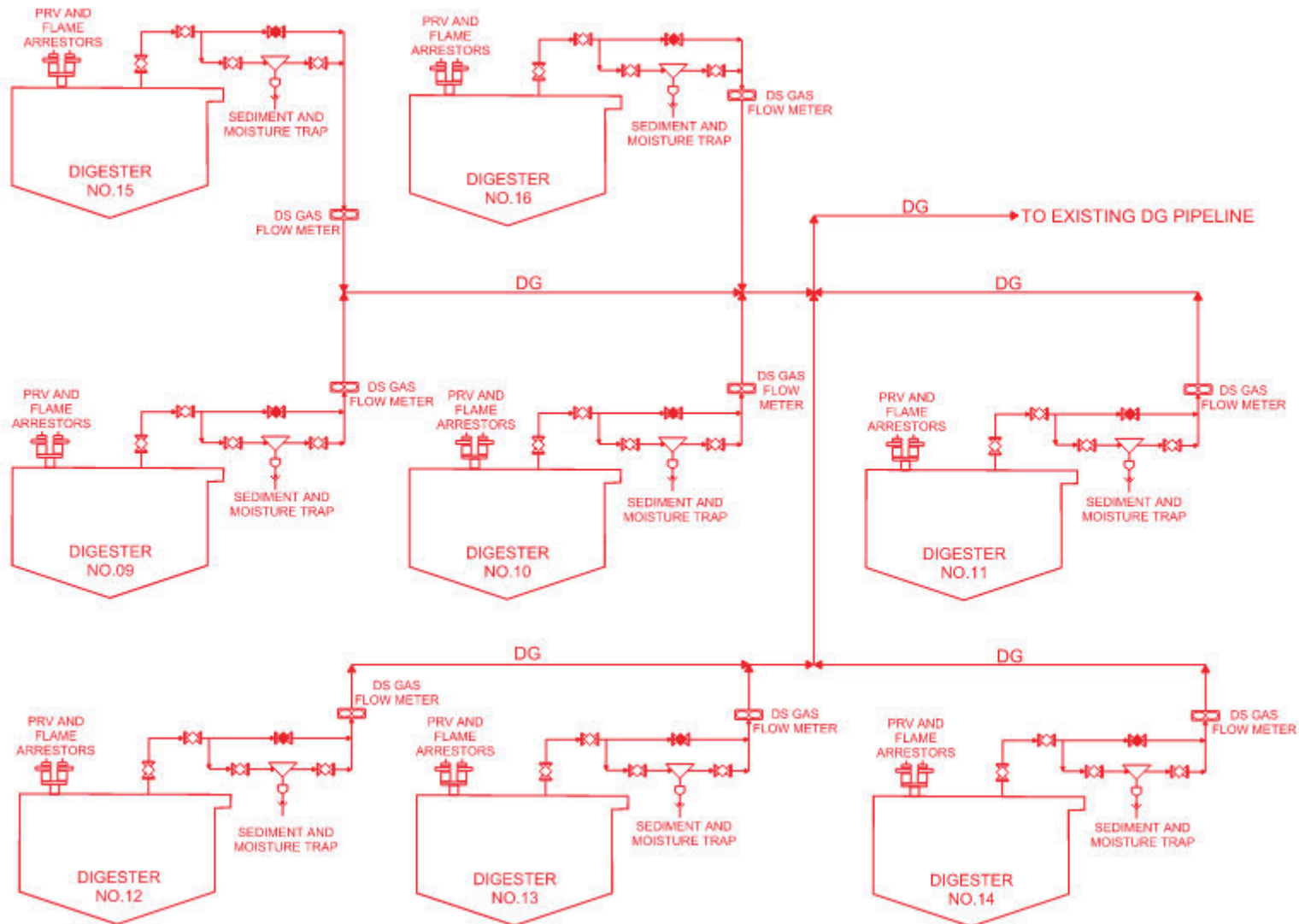
Figure 1-12 RWF Process Flow Diagram – Digester Gas
