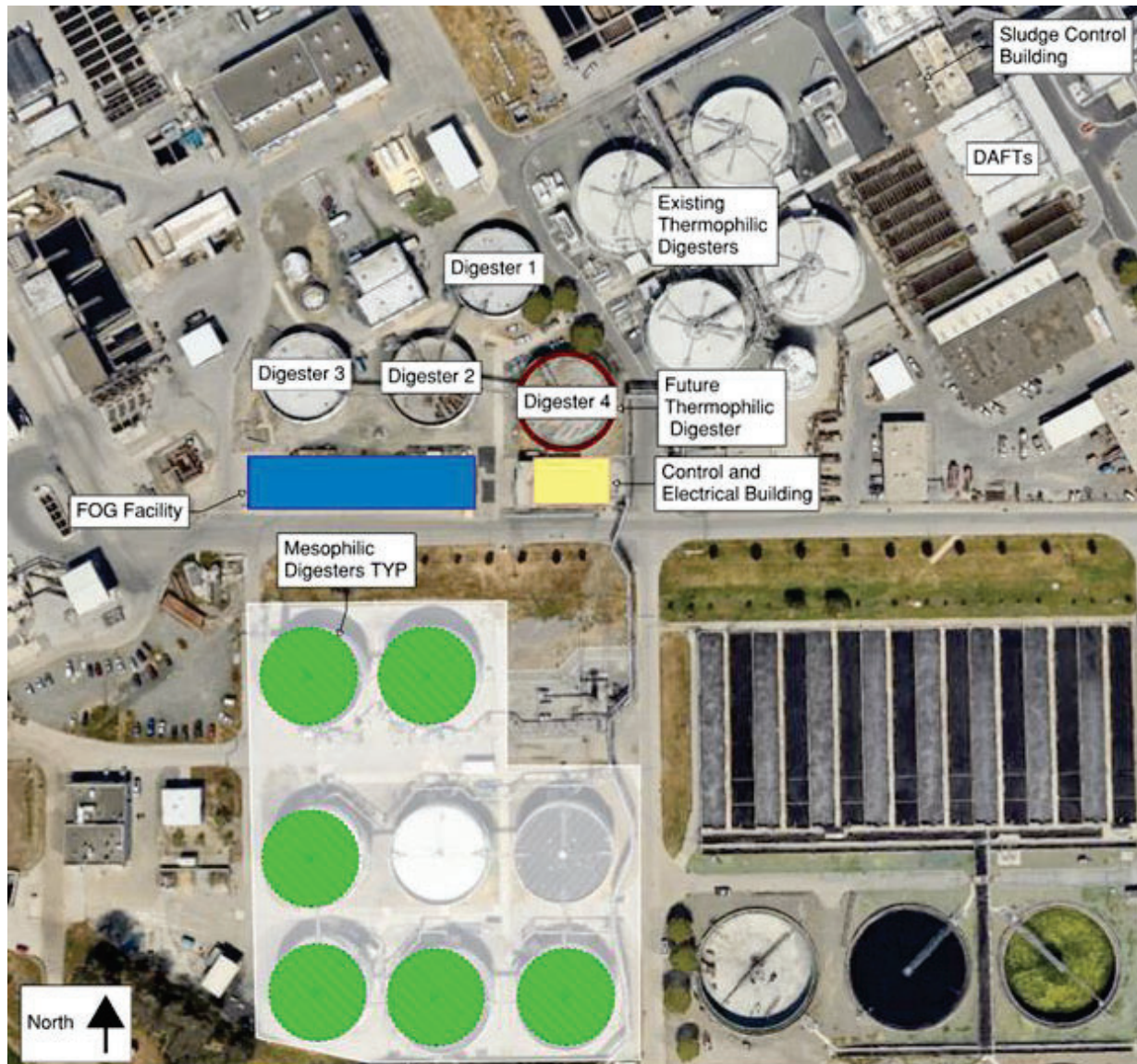
Figure 1-4 Indicative Design 1 – Base Alternative 2045 Layout
