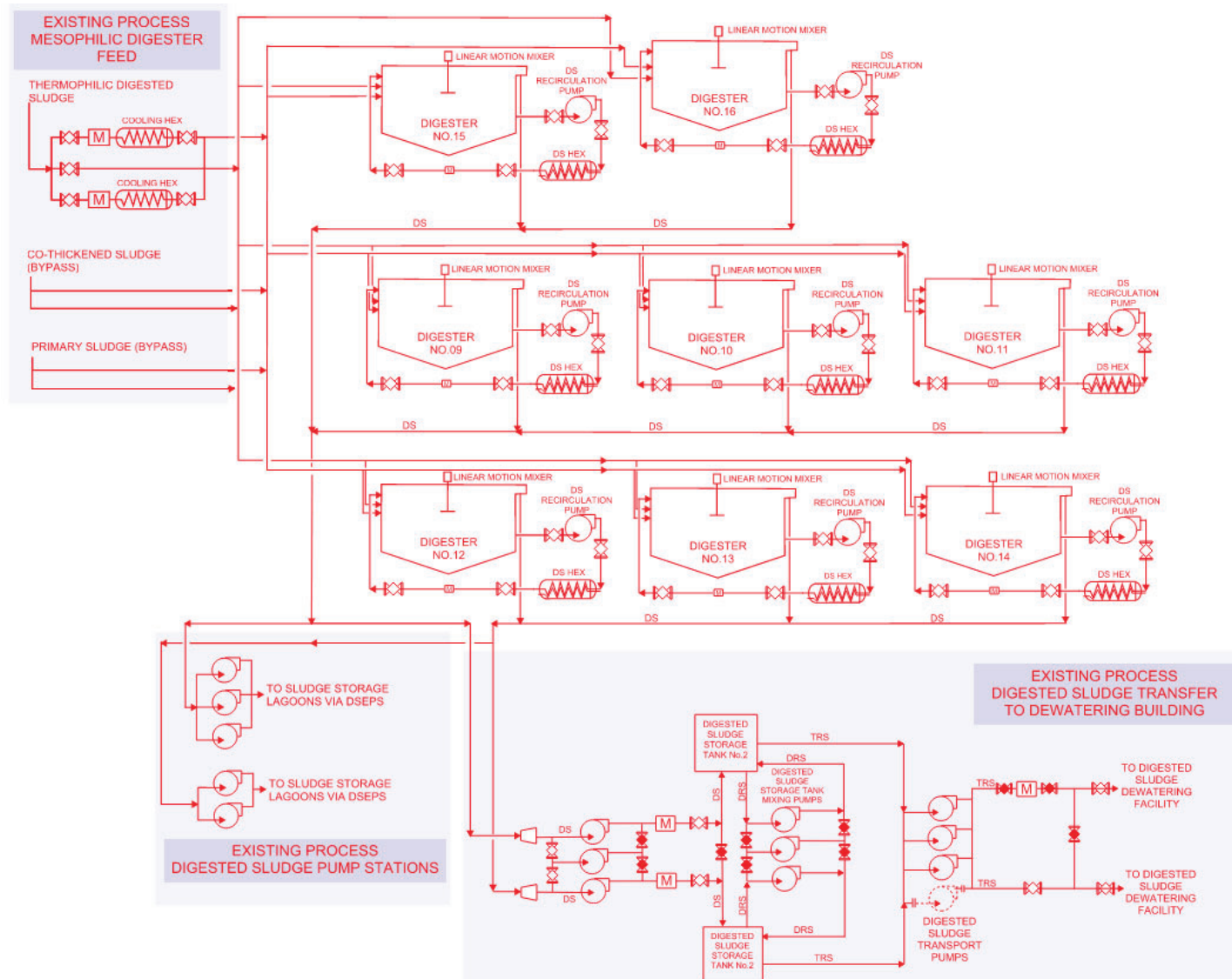
Figure 1-10 RWF Process Flow Diagram – Sludge Feed, Recirculation, and Transfer
