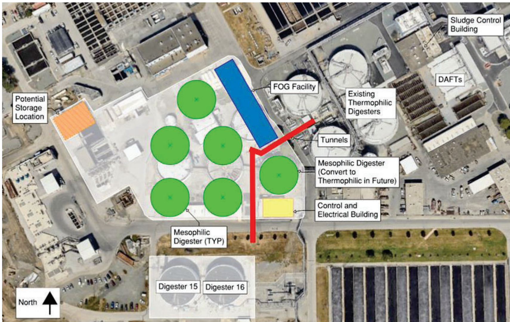
Figure 1-8 Indicative Design 3 – Alternative 2 2045 Layout
