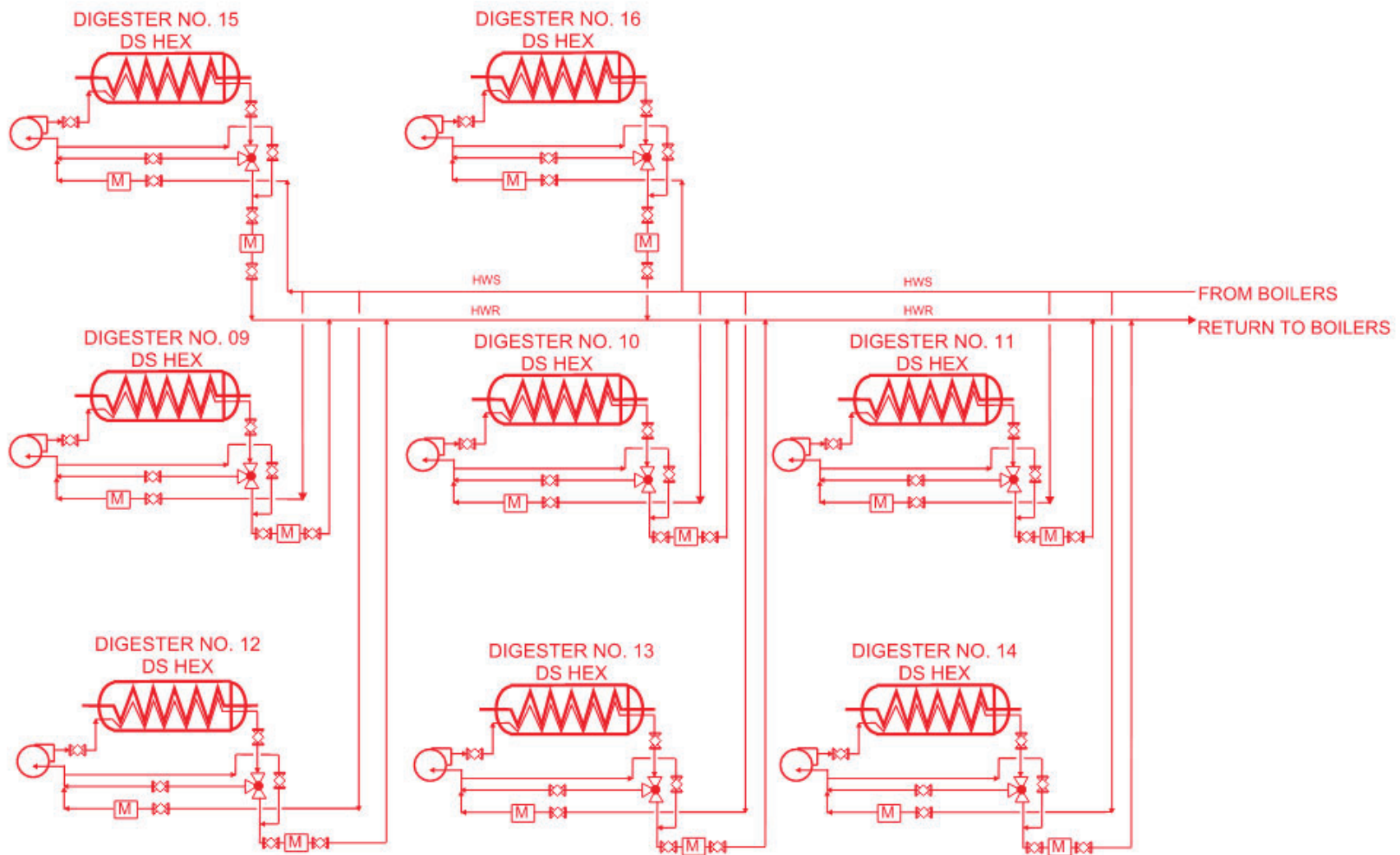
Figure 1-11 RWF Process Flow Diagram – Hot Water Loop
