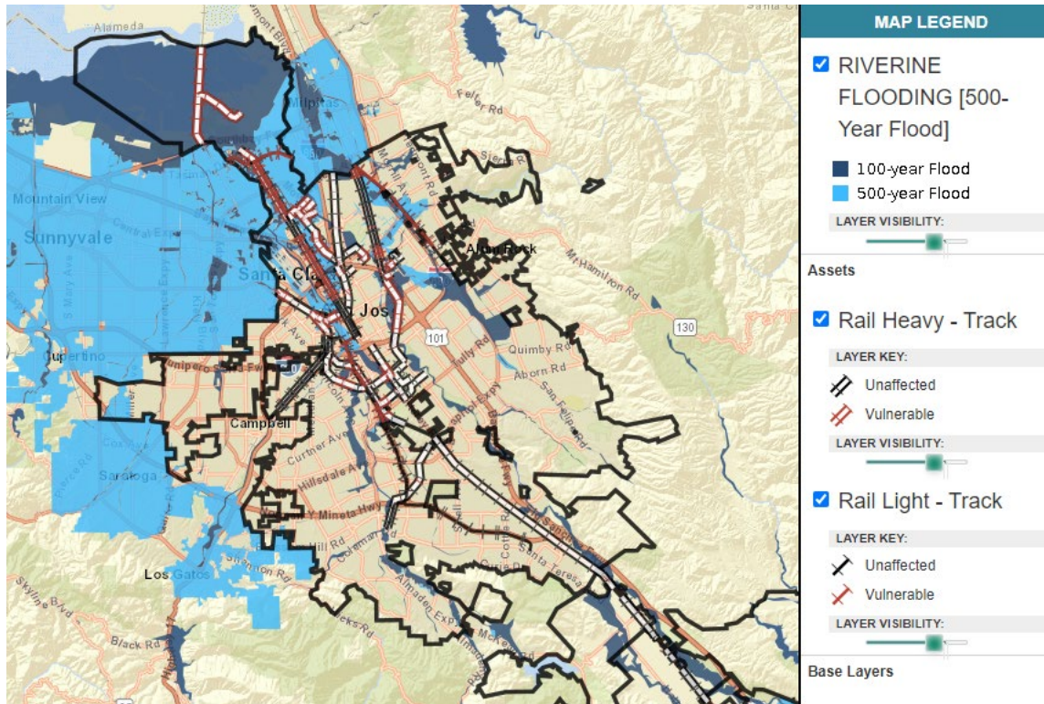
Figure 30. Light Rail &amp; Heavy Rail Exposure to Flooding (100-year and 500-year)
