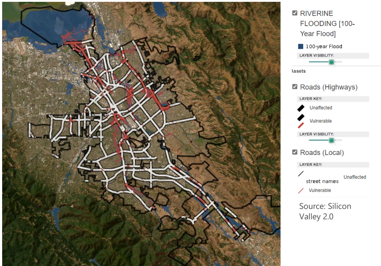
Figure 26: Roads &amp; Highways: Flooding Vulnerability
