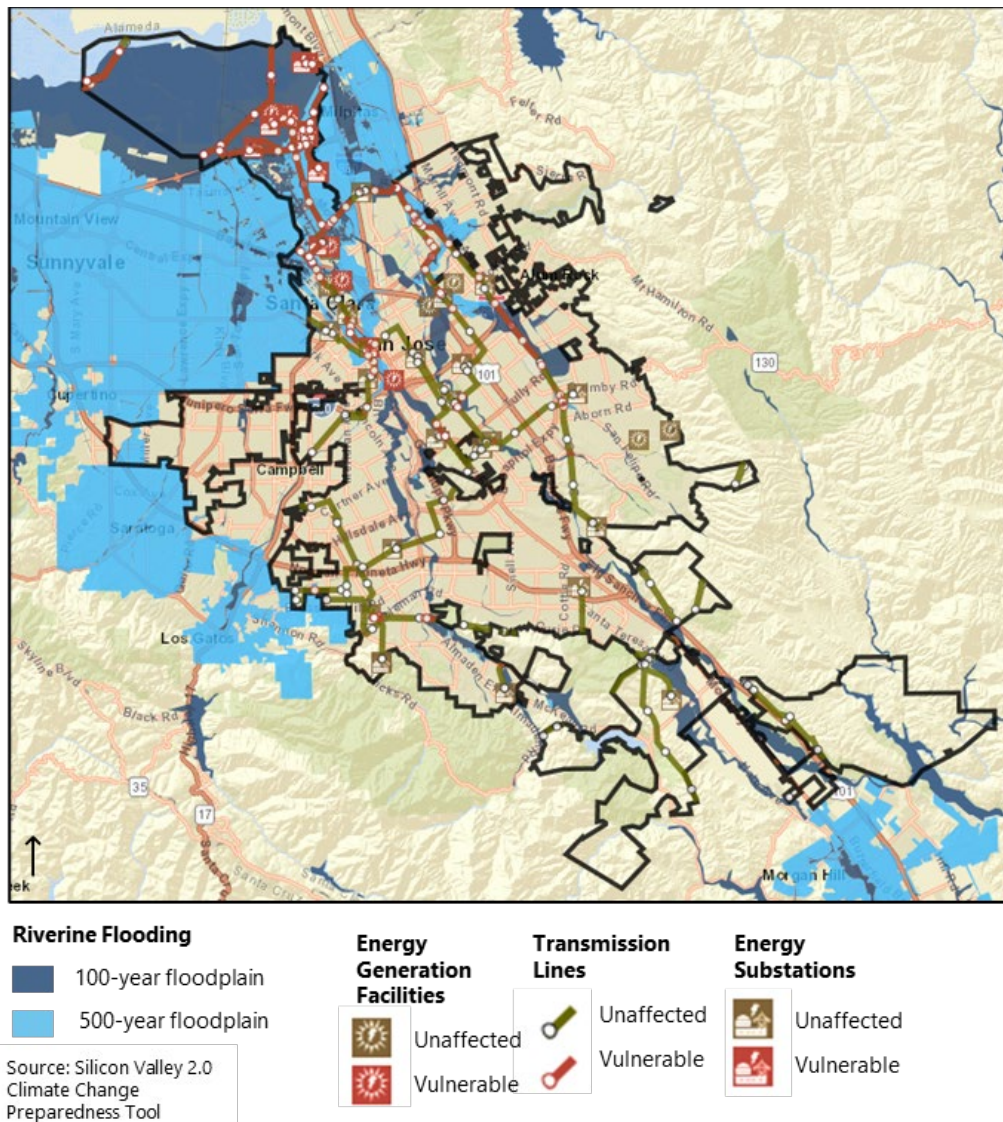
Figure 23. Energy Infrastructure Vulnerability to Flooding Based on Historical Floodplains
